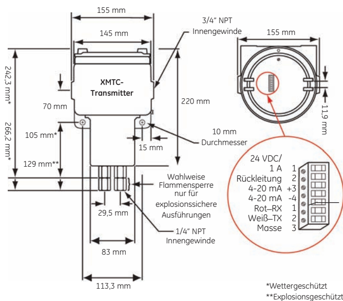
XMTC-Transmitter, Abmessungen
