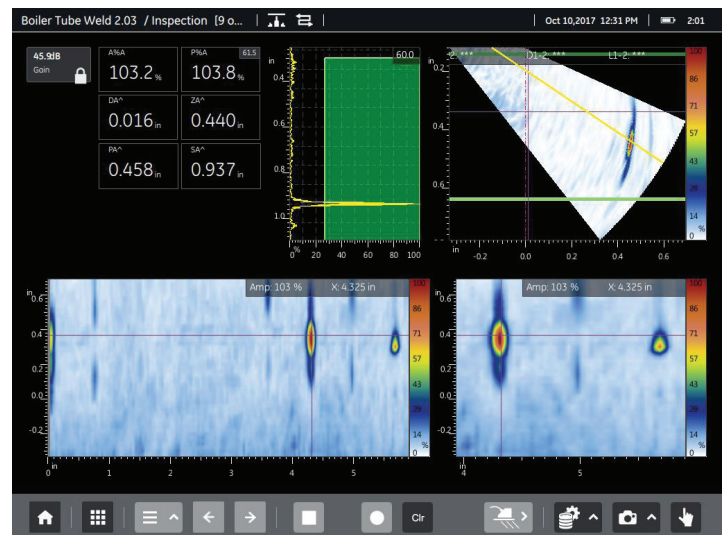
A, C and Sector Scans Show Weld Indications
