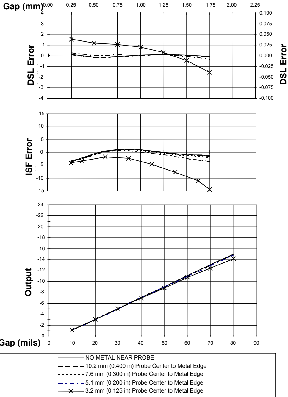
Figure 5: Effect of Flat Surface Side Clearance (4140 Material)
